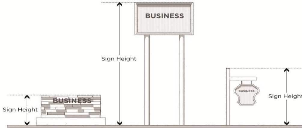
FIGURE 2-12: SIGN HEIGHT
